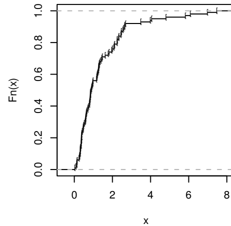
ecdf(lognorm100)
