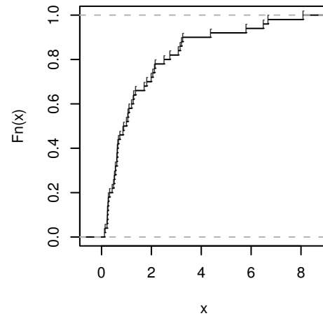
ecdf(lognorm50)
