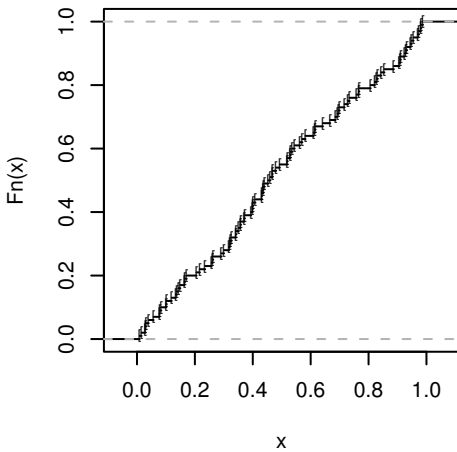
ecdf(unif100)
