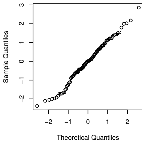
Normal Q-Q norm100
