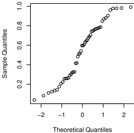
Normal Q-Q Plot unif50
