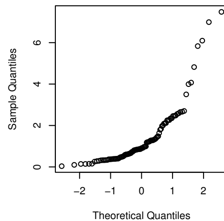
Normal Q-Q lognorm100
