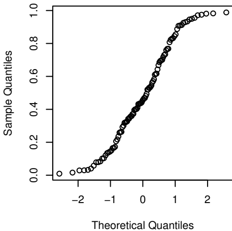
Normal Q-Q unif100
