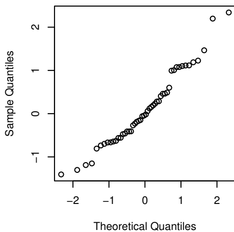
Normal Q-Q norm50
