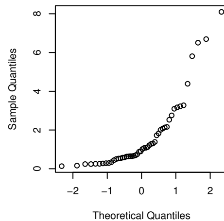
Normal Q-Q lognorm50
