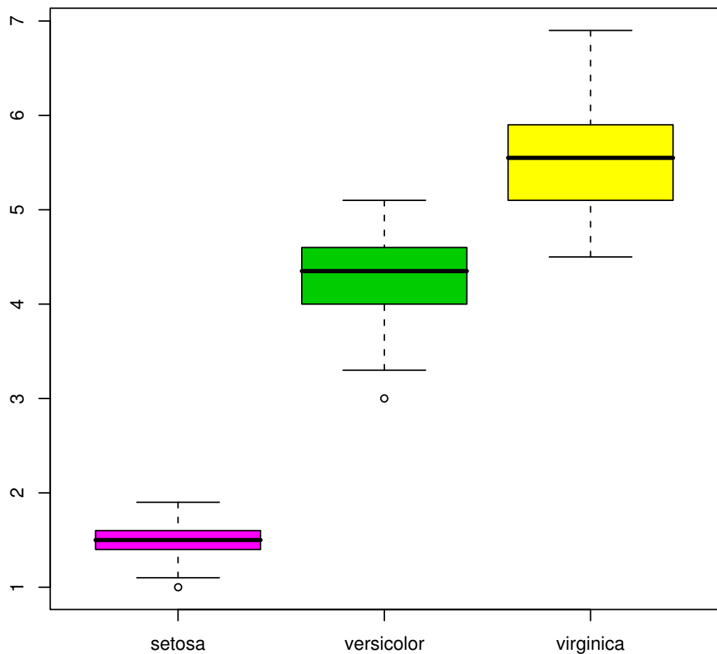
Petal Length
