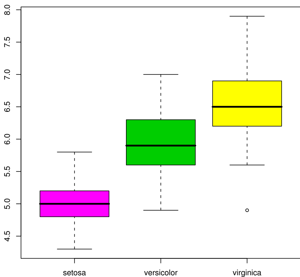
Sepal Length
