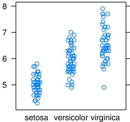
Sepal Length
