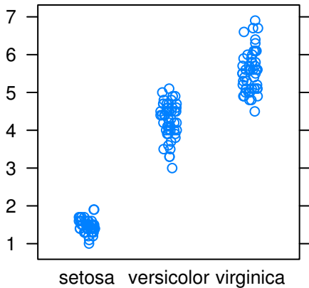
Petal Length
